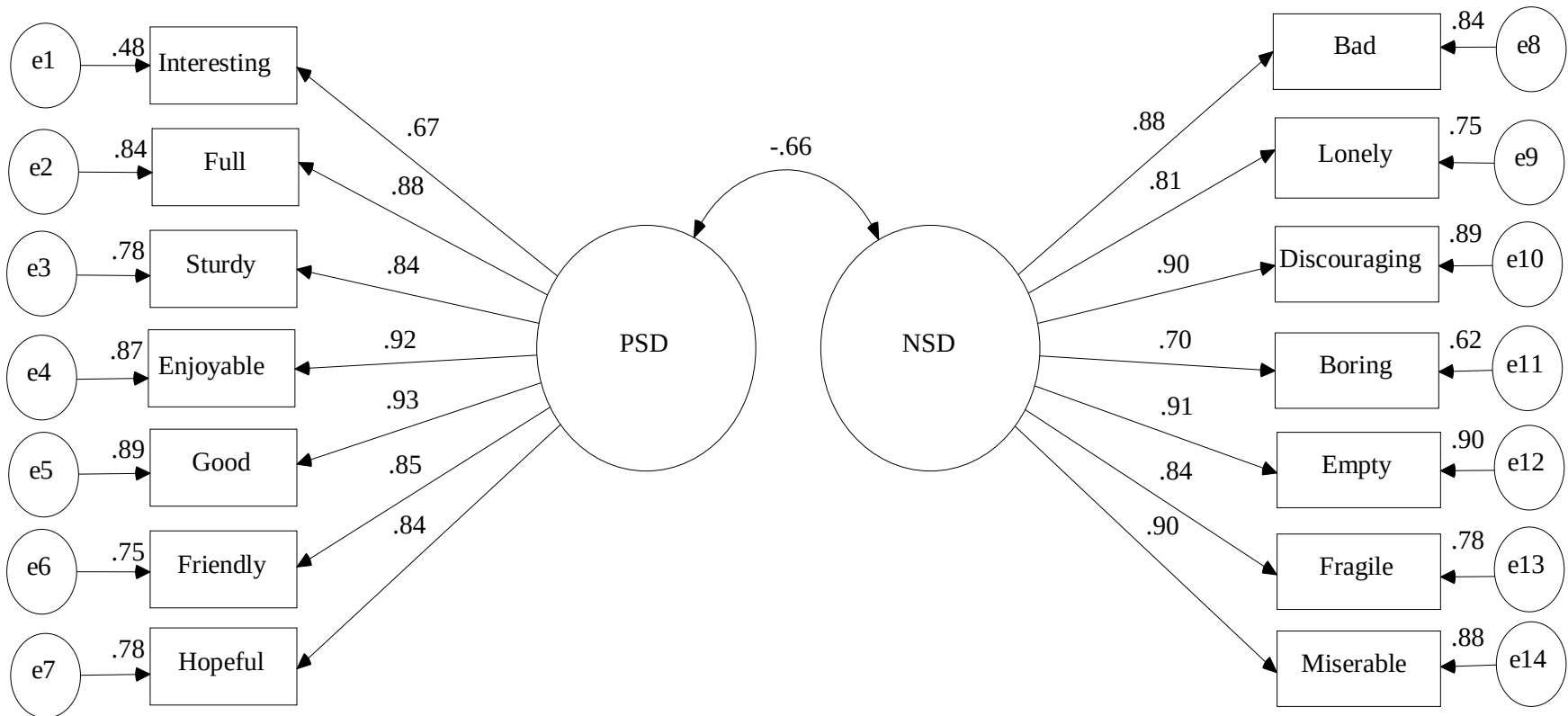
Figure 1. Parameter estimates for the oblique two-factor model of the PN-SMD. PSD = Positive Semantic Dimension; NSD = Negative Semantic Dimension. The items in the model appear in the sequence in which they were administered, beginning and ending with “Interesting” and “Hopeful,” respectively, for the PSD, and “Bad” and “Miserable,” also respectively, for the NSD.
